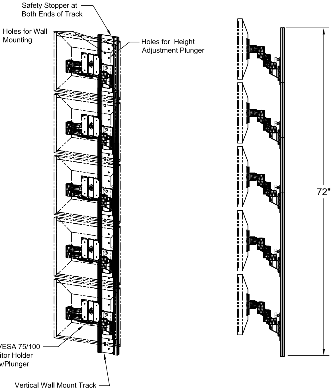
ISOMETRIC VIEW
