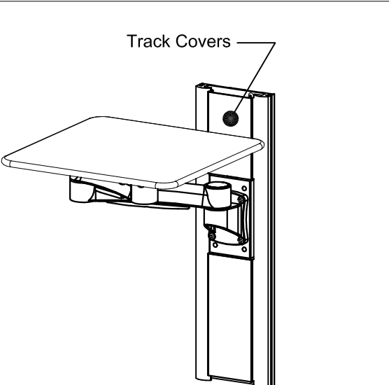
ISOMETRIC VIEW (with Covers) SCALE: ~1-1/2" = 1' - 0"
