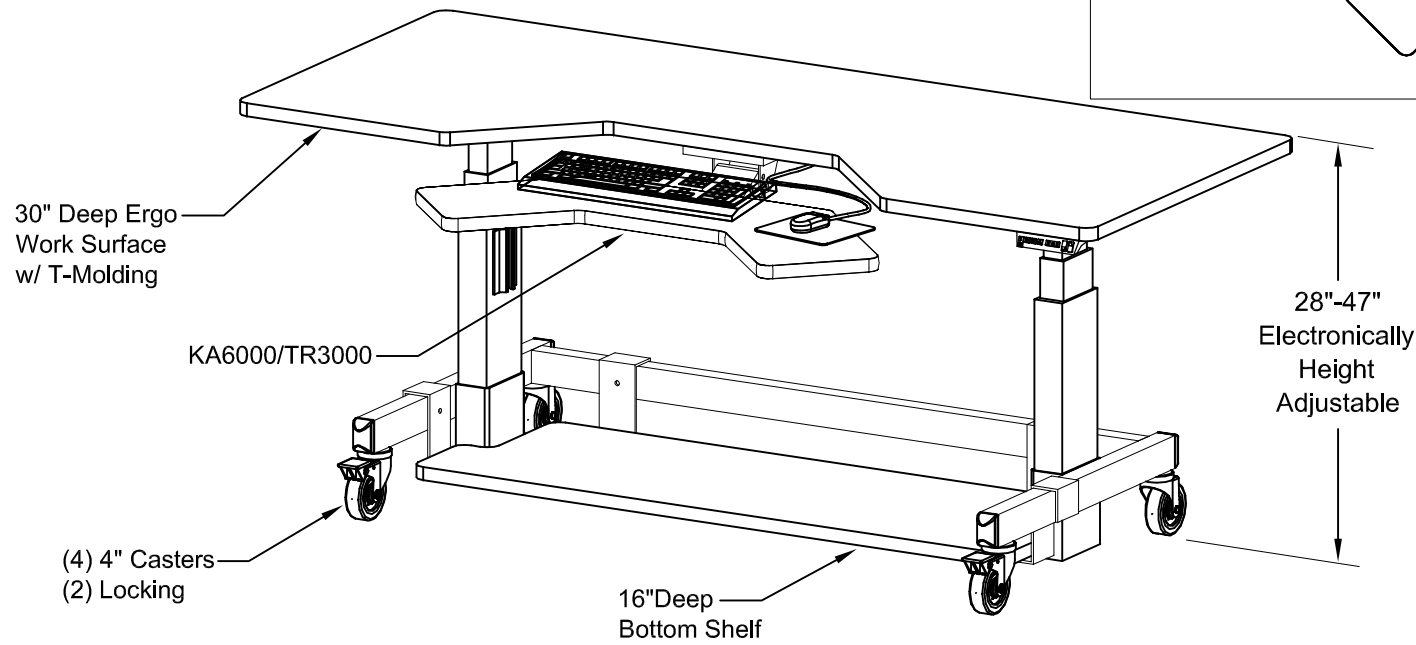
ISOMETRIC VIEW
