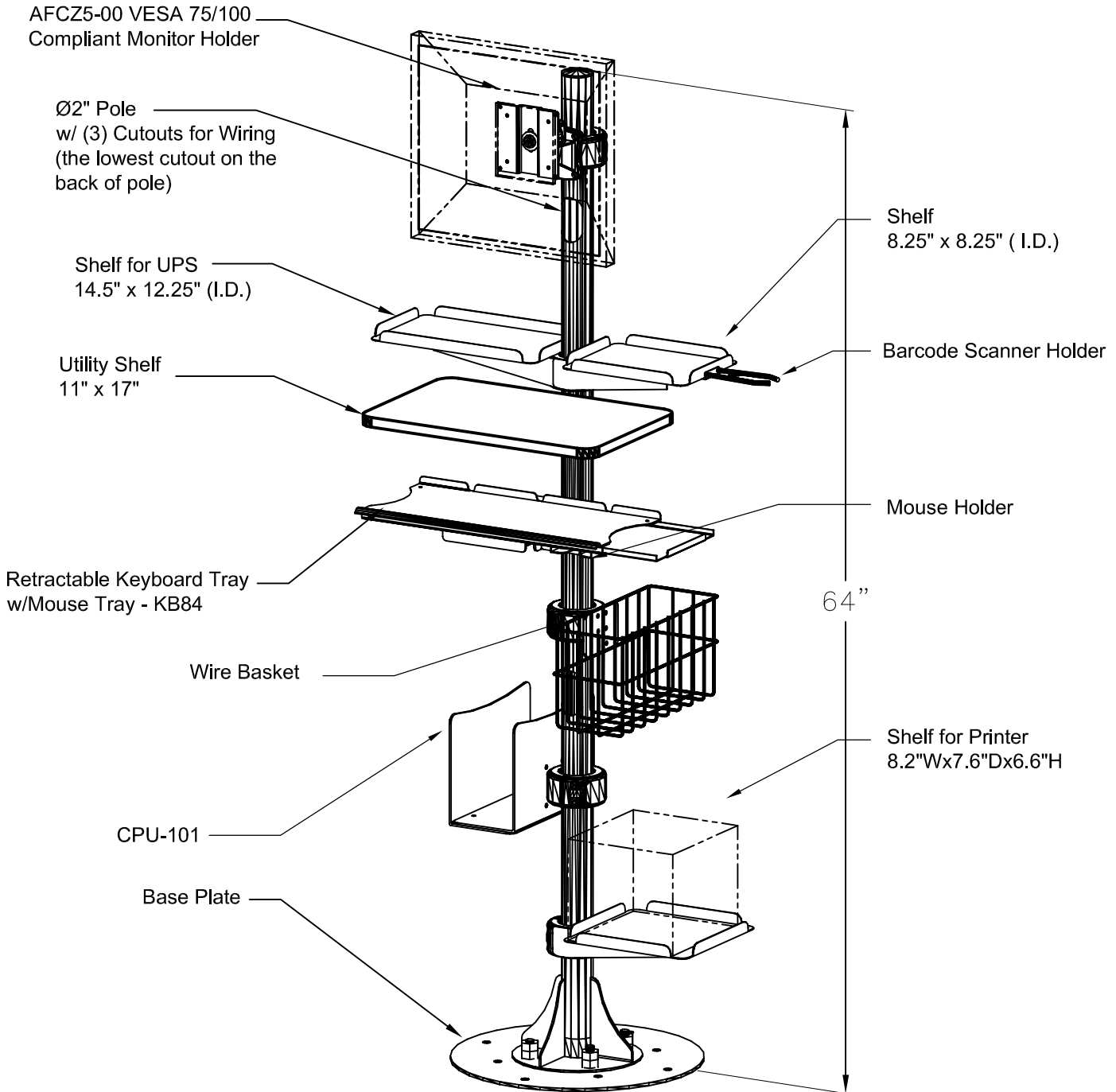
ISOMETRIC VIEW
