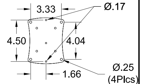
Standard Plate-Adapter Dimensions NOT TO SCALE
