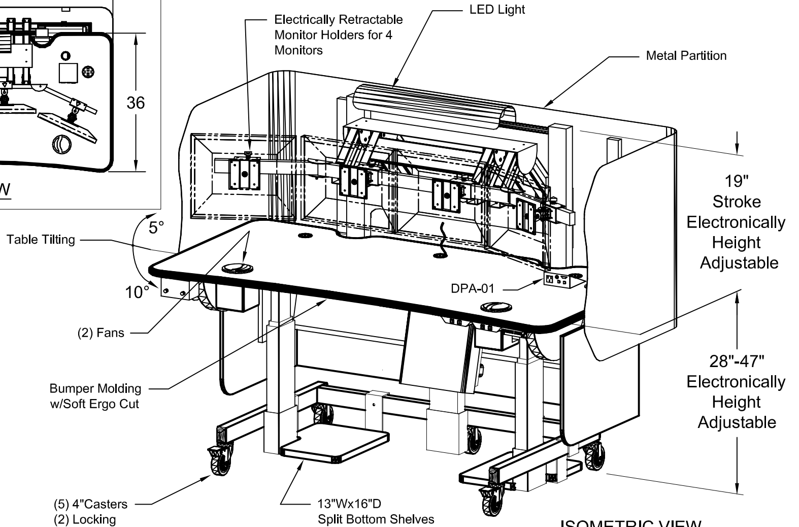
ISOMETRIC VIEW
